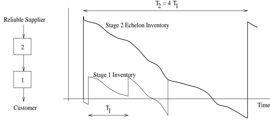
Figure 2: Typical Inventory Profile for Two-Stage Nested, (R, T) Policy
